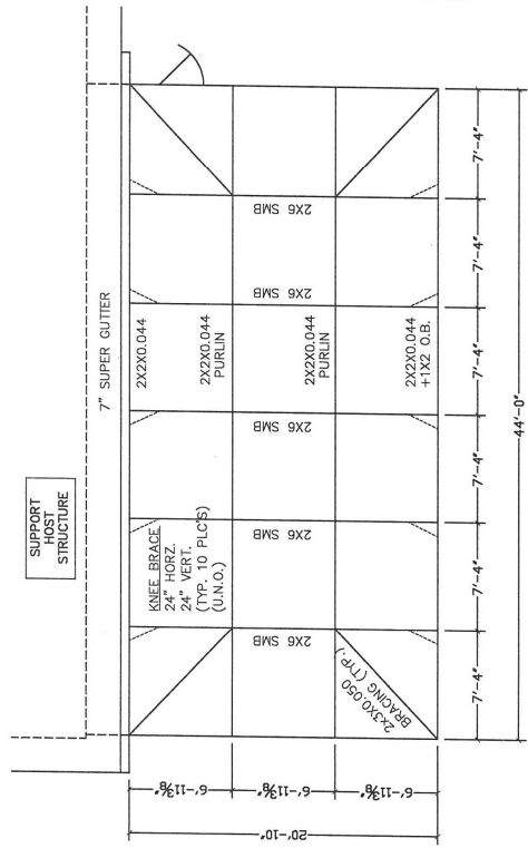
POOL ENCLOSURE PLAN
