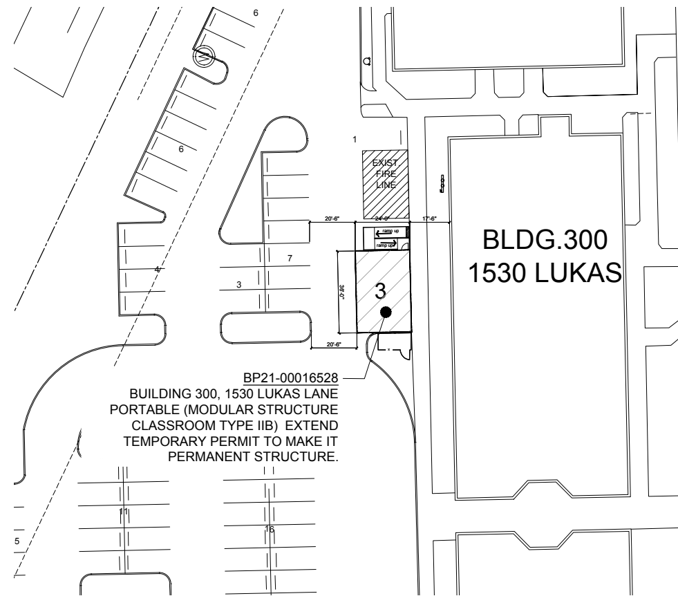
BUILDING 300 PORTABLE LOCATION SCALE: NTS
