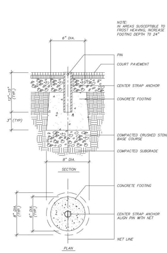
NOTE: PICKLEBALL COURTS TO BE CONSTRUCTED PER ARBAUSA PICKLEBALL CONSTRUCTION MANUAL. 3 | PICKLEBALL NET CENTER STRAP ANCHOR NTS. PROVIDED BY NEY SPORTS CONSTRUCTION
