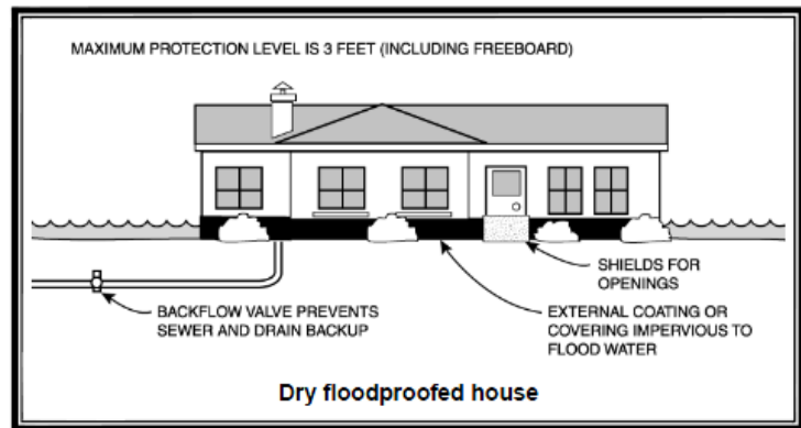
Figure 34: Dry Floodproofing
