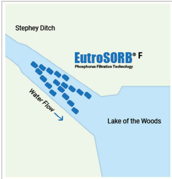
EutroSORB F filters strategically deployed in Stephey Ditch to intercept free reactive phosphorus and treat the water before it continues downstream.
