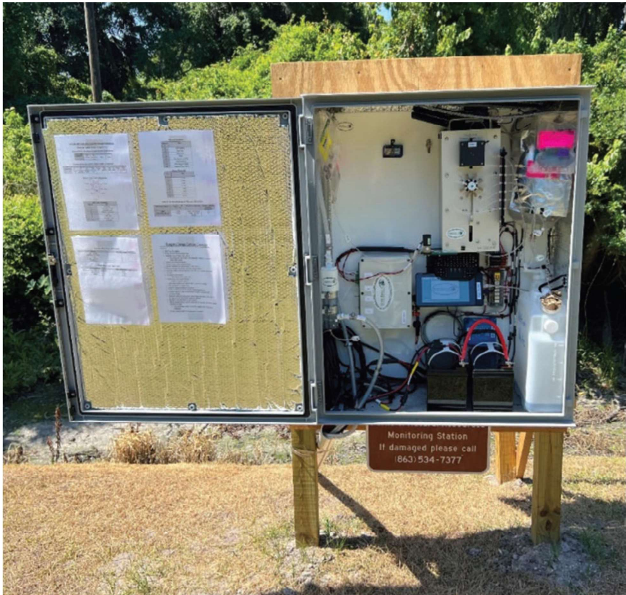
Figure 4. NuLAB Continuous Monitoring System
