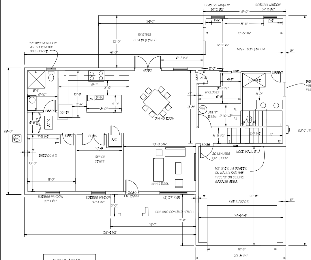
FIRST FLOOR
